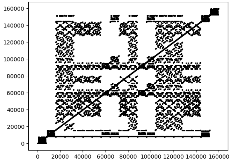
Figure 19: a_{20}(n) for n \in \{1, 2, \dots, 20^4\} .
