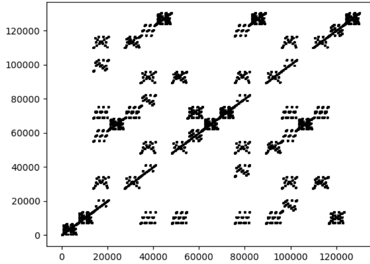
Figure 18: a_{19}(n) for n \in \{1, 2, \dots, 19^4\} .
