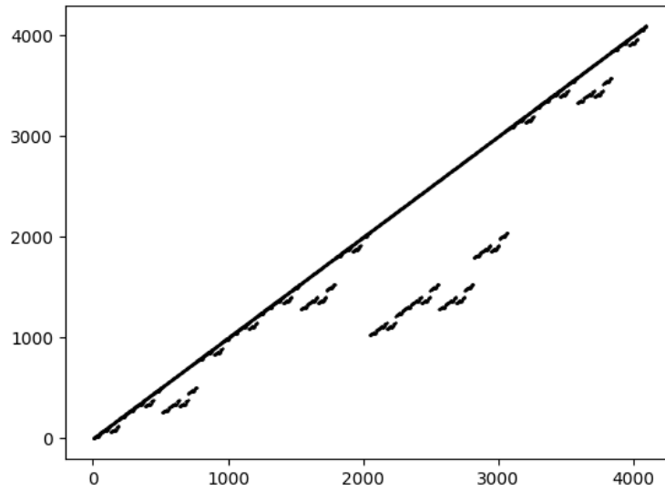
Figure 3: a_4(n) for n \in \{1, 2, \dots, 4^6\} .
