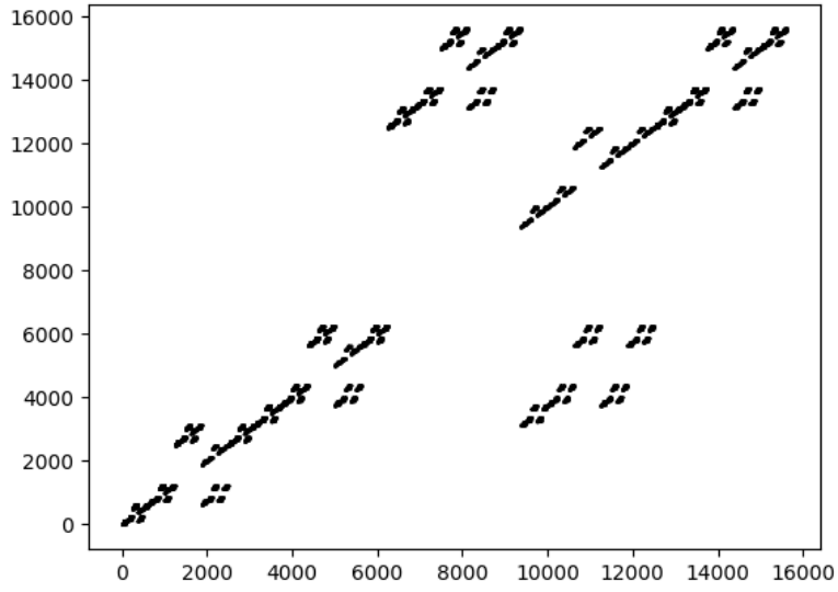
Figure 4: a_5(n) for n \in \{1, 2, \dots, 5^6\} .
