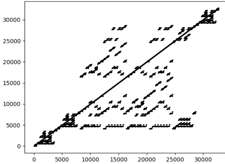
Figure 7: a_8(n) for n \in \{1, 2, \dots, 8^5\} .
