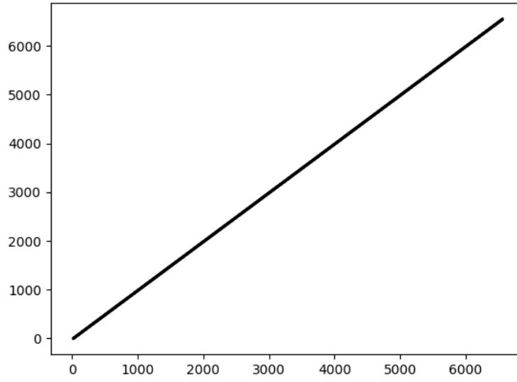
Figure 2: a_3(n) for n \in \{1, 2, \dots, 3^8\} .
