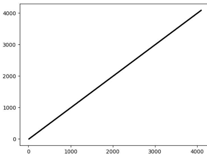
Figure 1: a_2(n) for n \in \{1, 2, \dots, 2^{12}\} .
