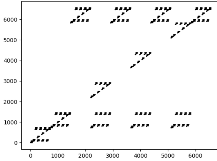
Figure 8: a_9(n) for n \in \{1, 2, \dots, 9^4\} .
