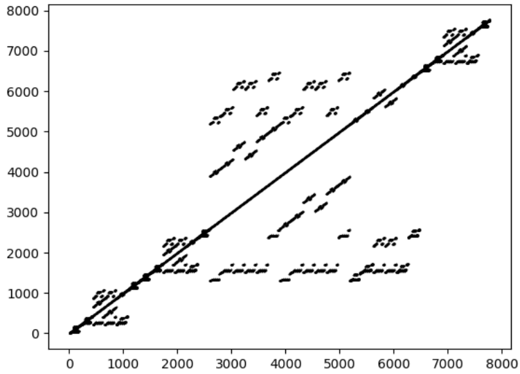
Figure 5: a_6(n) for n \in \{1, 2, \dots, 6^5\} .
