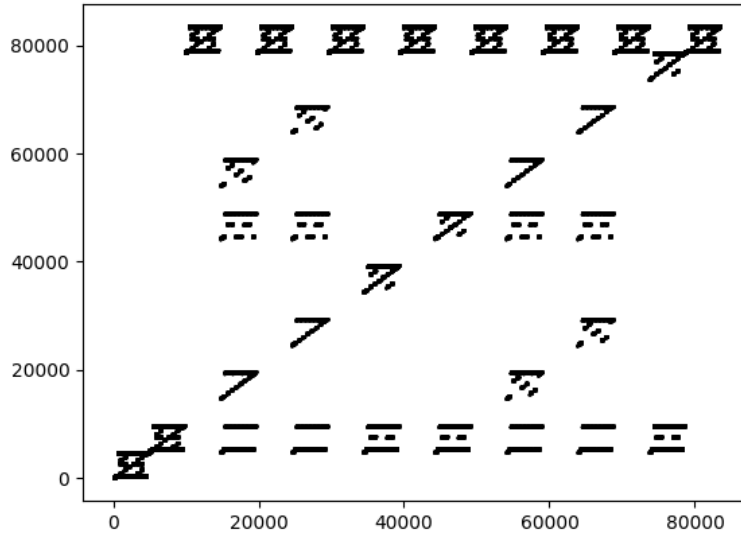
Figure 16: a_{17}(n) for n \in \{1, 2, \dots, 17^4\} .
