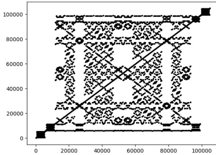
Figure 17: a_{18}(n) for n \in \{1, 2, \dots, 18^4\} .
