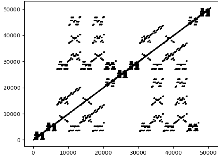
Figure 14: a_{15}(n) for n \in \{1, 2, \dots, 15^4\} .
