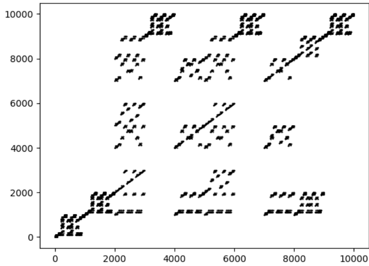
Figure 9: a_{10}(n) for n \in \{1, 2, \dots, 10^4\} .
