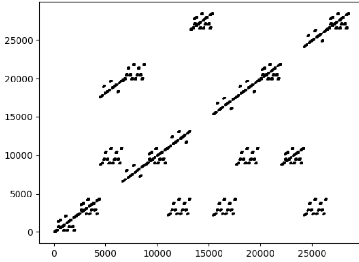
Figure 12: a_{13}(n) for n \in \{1, 2, \dots, 13^4\} .
