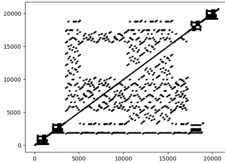
Figure 11: a_{12}(n) for n \in \{1, 2, \dots, 12^4\} .
