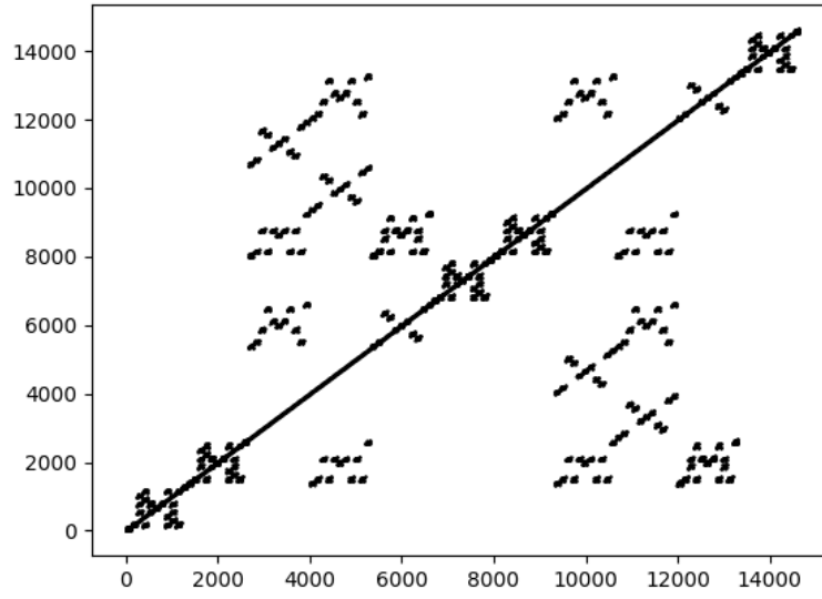
Figure 10: a_{11}(n) for n \in \{1, 2, \dots, 11^4\} .
