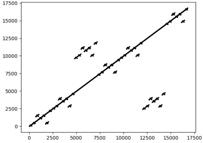
Figure 6: a_7(n) for n \in \{1, 2, \dots, 7^5\} .
