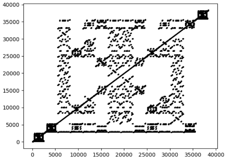
Figure 13: a_{14}(n) for n \in \{1, 2, \dots, 14^4\} .
