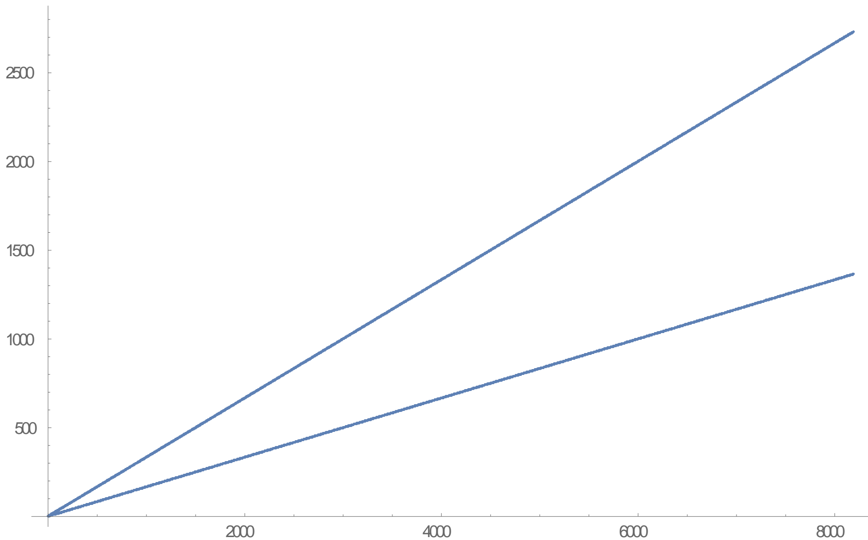
Scatter plot of first 2^{13} terms of A289777
